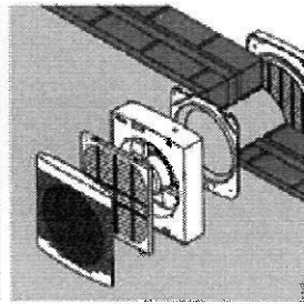
9" & 12" Wall Mounting
