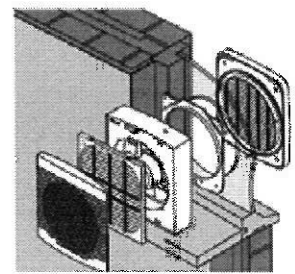
9" & 12" Window Mounting
