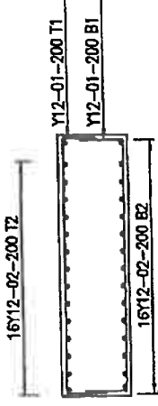
SECTION A-A SCALE 1:50
