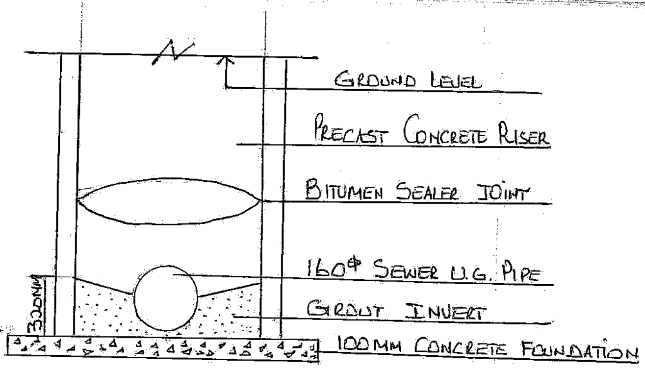
PRECAST MANHOLE OVER NEW SEWER LINE
