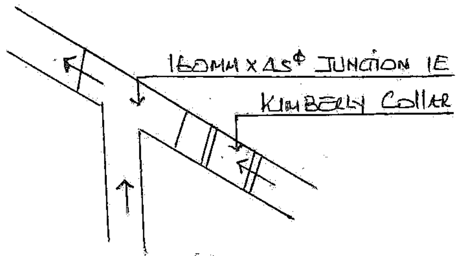
CHANNEL AND BENCHING DETAILS
