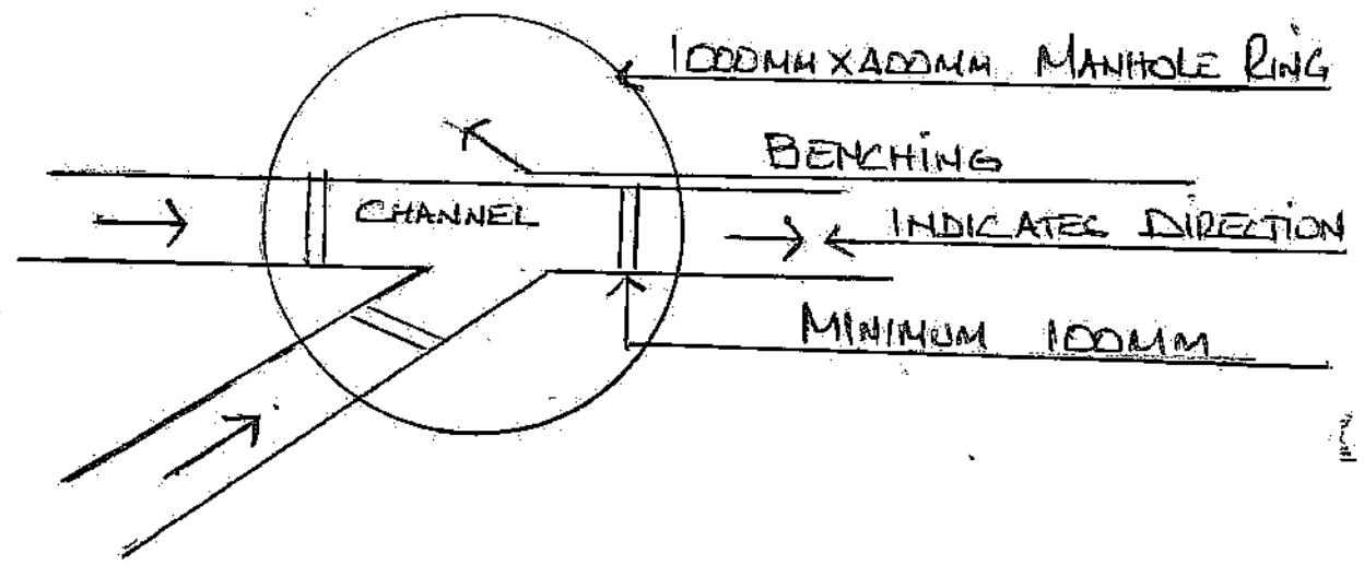
CHANNEL AND BENCHING DETAILS
