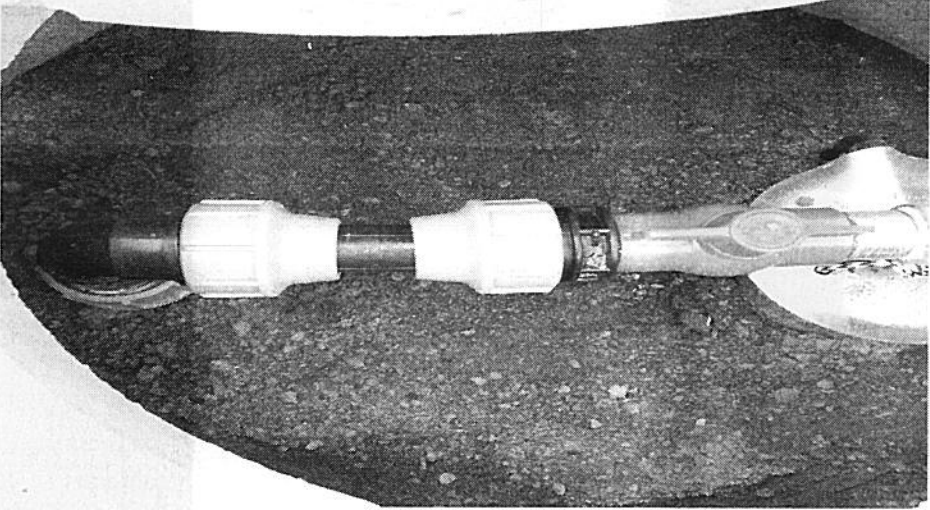
Connection piece between borehole and water supply pipe
