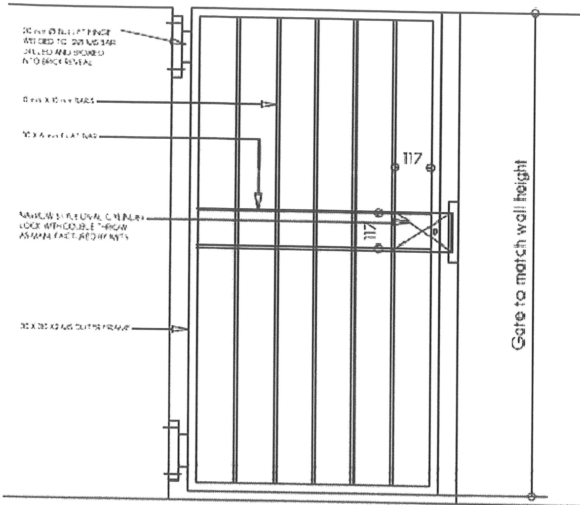
1:10 TYPICAL GATE DETAIL
