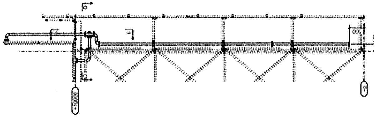
Overflo & Drain 65NB 1600/3
