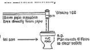
Model: Watera 106T 25mm BSP, exposed, lever operated, chrome, toilet flushing valve with top entry flush pipe.
