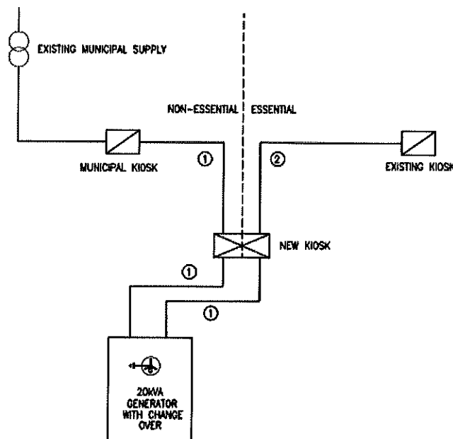
Figure 2: Generator Schematic
