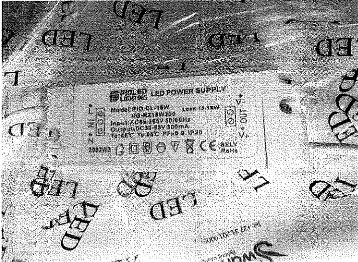
LED power supply, model PIO-CL-18w. Load: 13-18 w (PIOLED)
