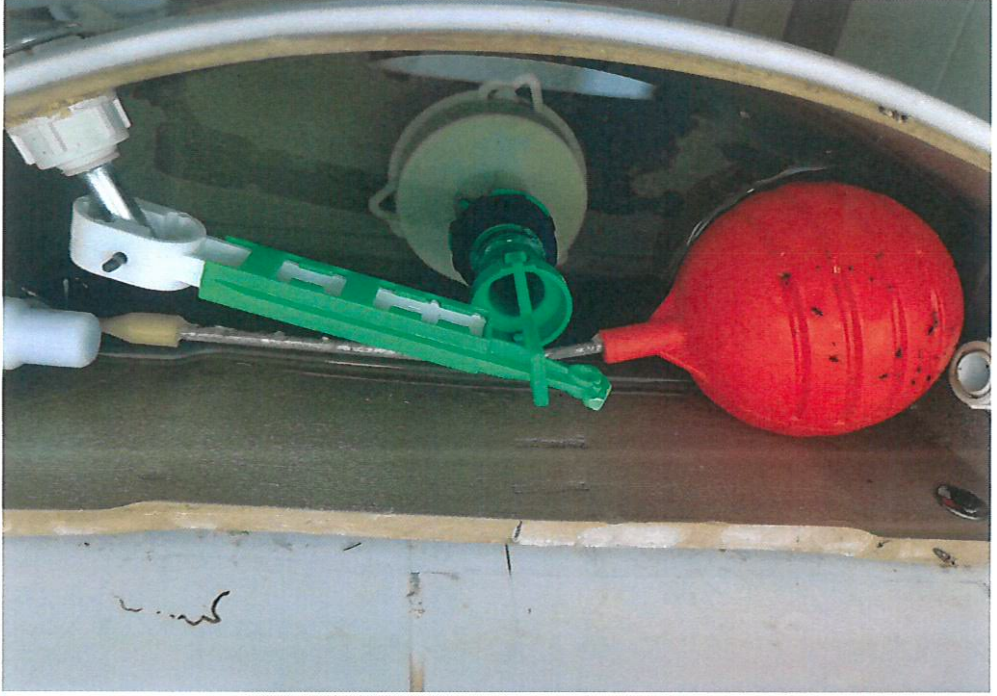
Water Inlets Toilet 30 Ball Valve (side view)
