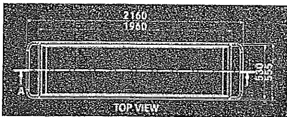
F-BTS - standard body tray dimensions
