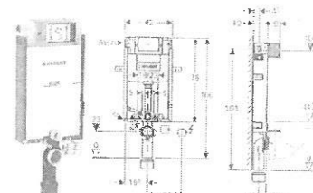
OMEGA KOMBIFIX CISTERN 106 CM FRONT ACTUATION ONLY Height to the top: 106 cm, Width: 42 cm 110.020.00.1
