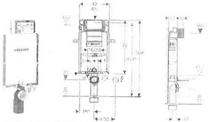
EBERIT SIGMA KOMBIFIX CISTERN 12 CM FOR WALL-HUNG APPLICATIONS Height to the top: 108 cm, Width: 42 cm, Depth: 12 cm 110.350.00.5
