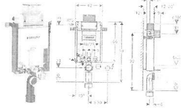
OMEGA KOMBIFIX CISTERN 98 CM TOP & FRONT ACTUATION Height to the top: 98 cm, Width: 42 cm 110.011.00.1
