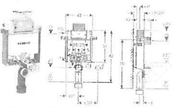
OMEGA KOMBIFIX CISTERN 82 CM TOP & FRONT ACTUATION Height to the top: 82 cm, Width: 42 cm 110.001.00.1
