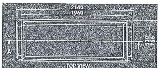
F-BTO – Obese body tray dimensions
