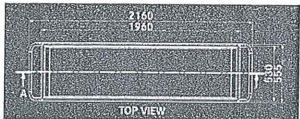
F-BTS – standard body tray dimensions
