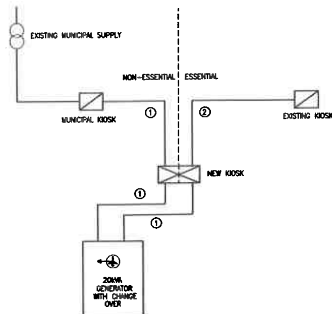
Figure 2: Generator Schematic
